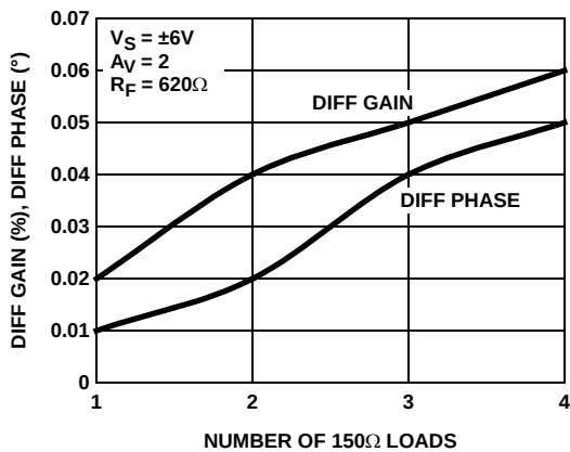
FIGURE 31. DIFFERENTIAL GAIN/PHASE
