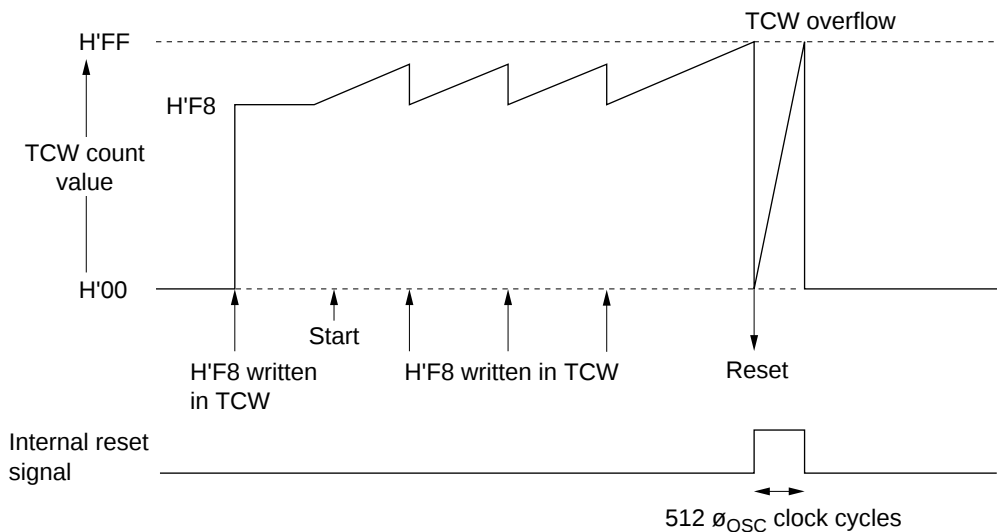
Figure 9-17 Typical Watchdog Timer Operations (Example)
