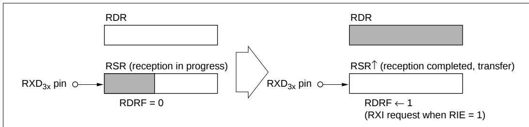
Figure 10-7 (a) RDRF Setting and RXI Interrupt
