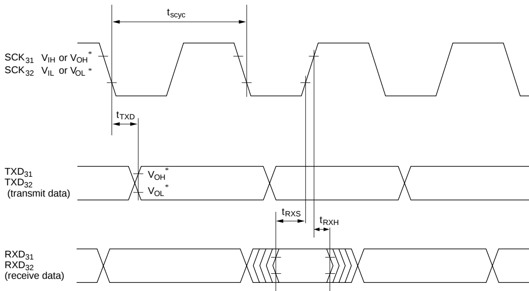
Figure 15-6 SCK3 Input Clock Timing
