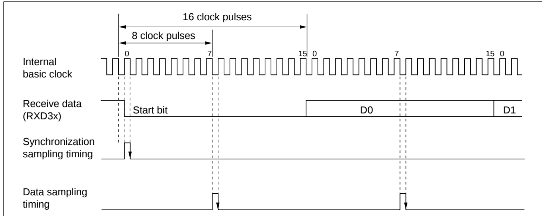
Figure 10-26 Receive Data Sampling Timing in Asynchronous Mode
