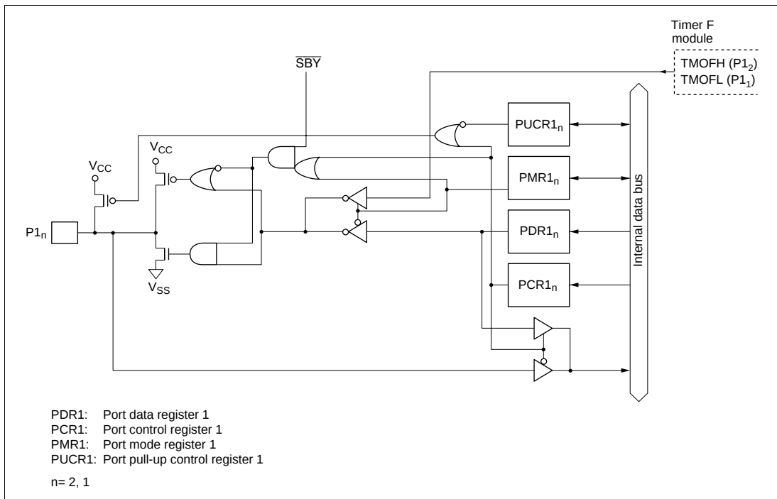
Figure C-1 (c) Port 1 Block Diagram (Pin P1 n , P1 1 )
