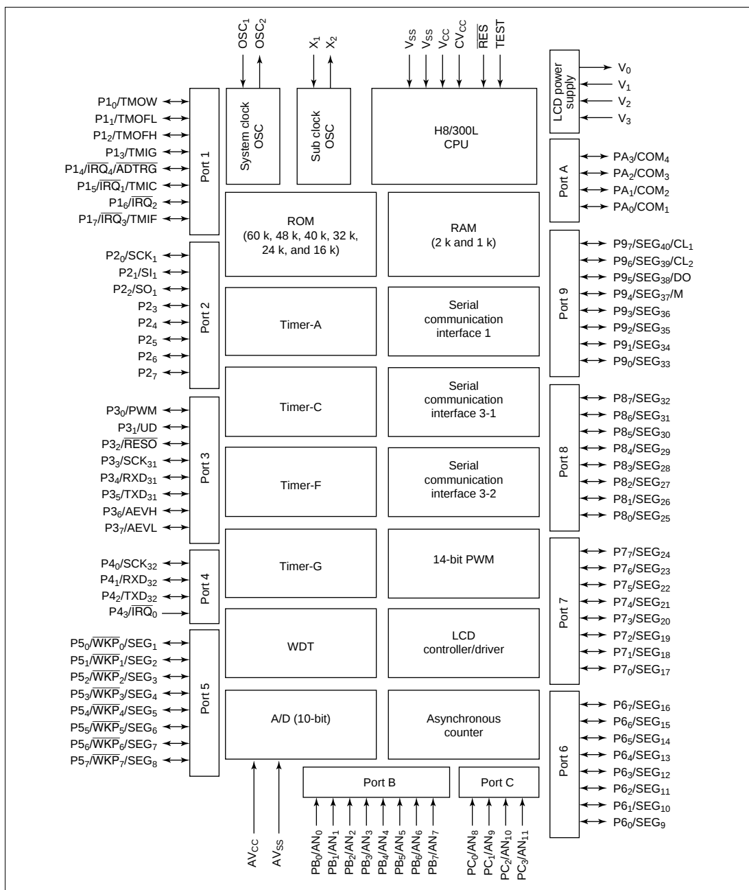
Figure 1-1 Block Diagram
