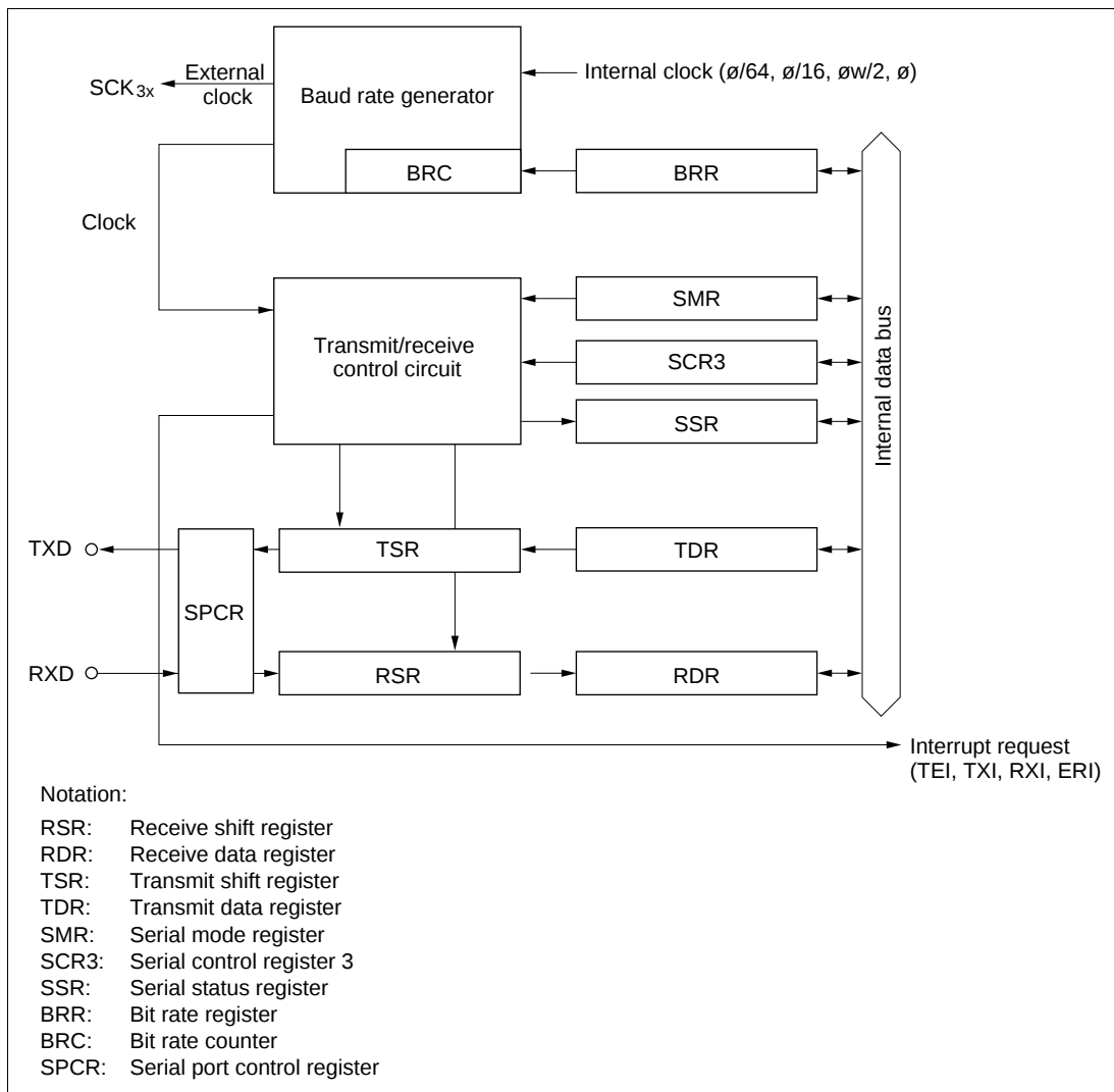
Figure 10-6 SCI3 Block Diagram
