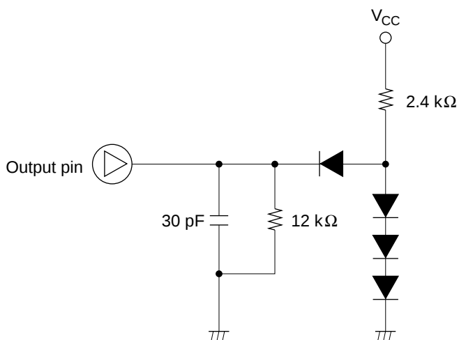
Figure 15-9 Output Load Condition
