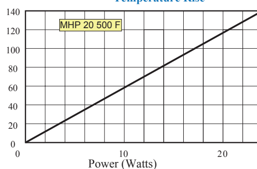
Temperature Rise
