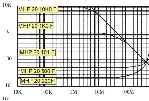
Frequency Characteristics
