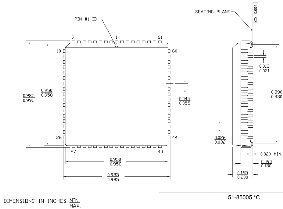
Figure 18. 68-pin Plastic Leaded Chip Carrier
