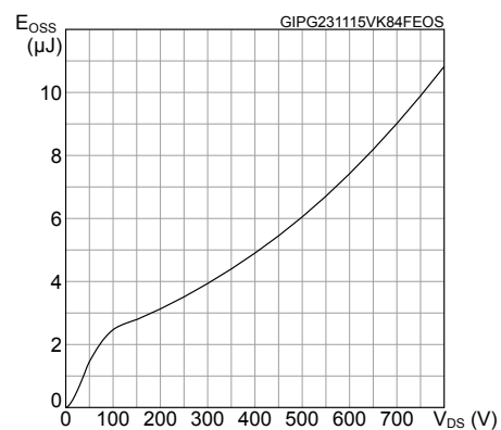
Figure 13. Typical output capacitance stored energy
