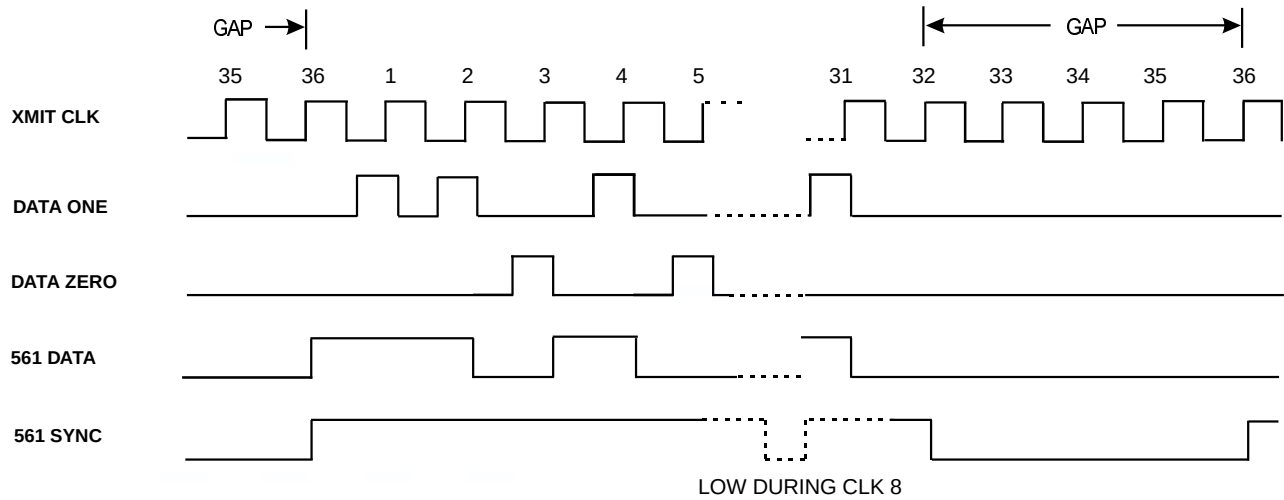
DATA TRANSMISSION - EXAMPLE PATTERN
