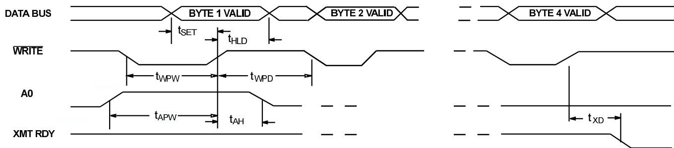
TRANSMITTER OPERATION
