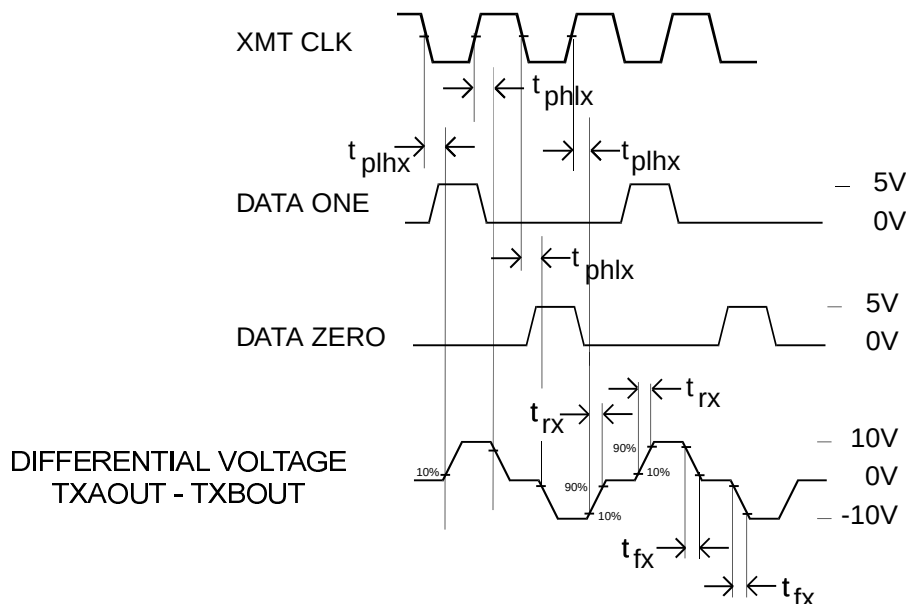
LINE DRIVER OUTPUTS
