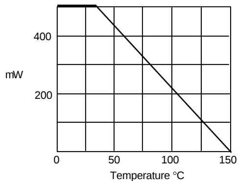
Figure 2 - Derating Curve
