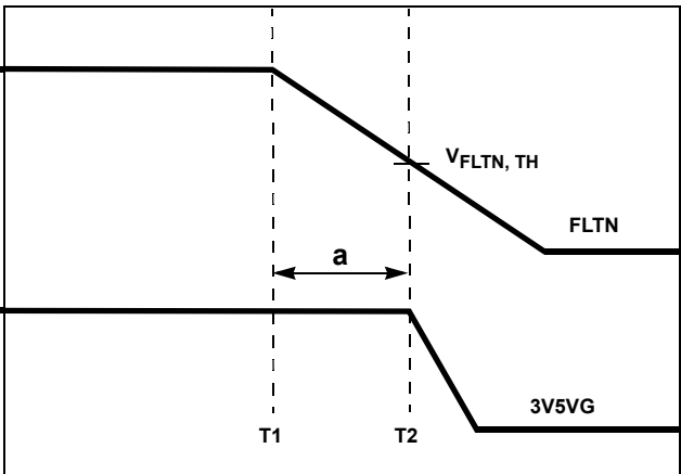
FIGURE 12. TIMING DIAGRAM
