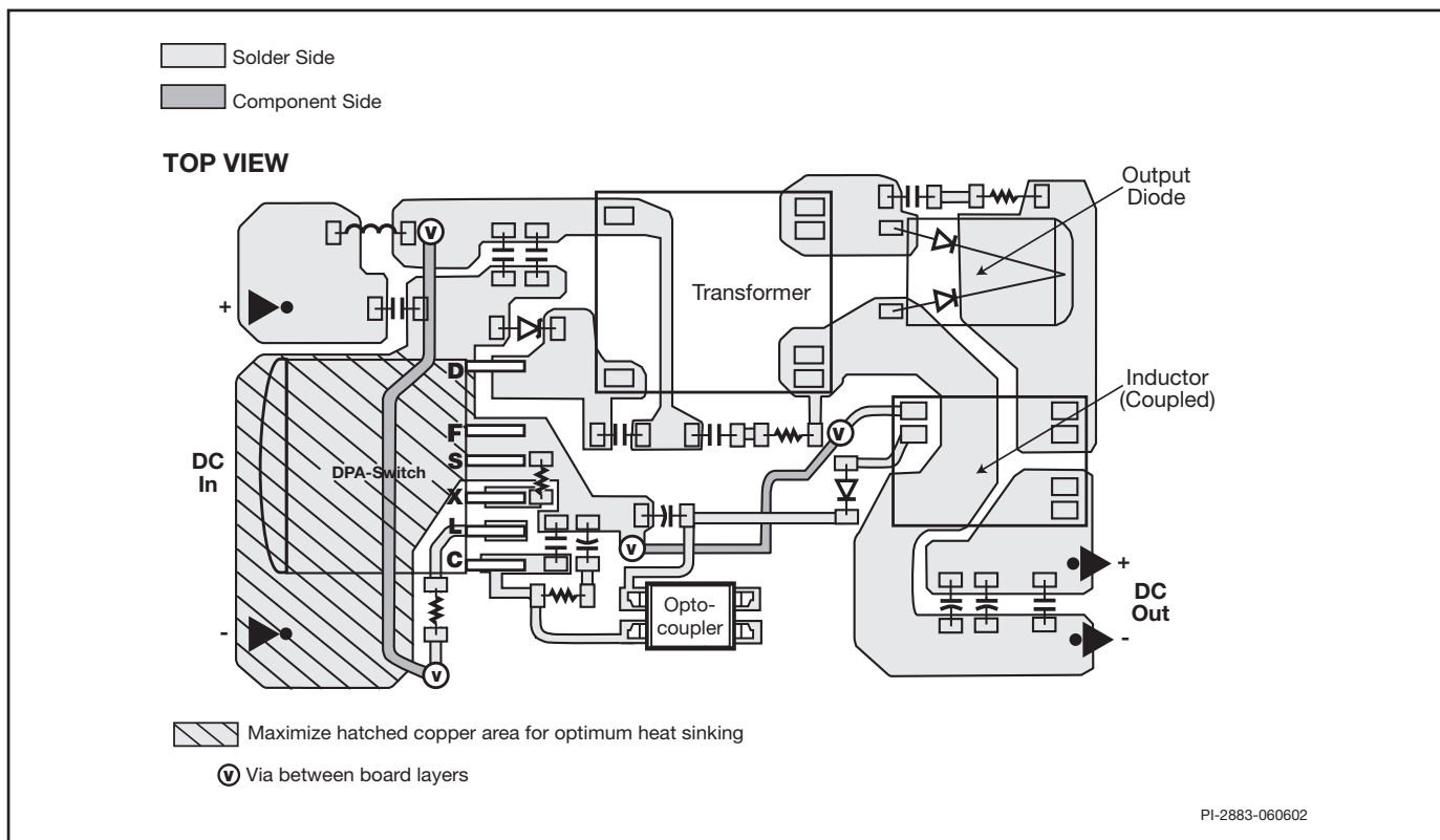
Figure 28. Layout Considerations for DPA-Switch Using R Package.
