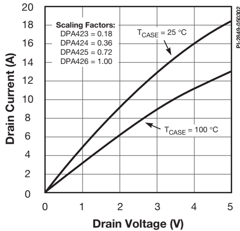
Figure 48. Output Characteristics.
