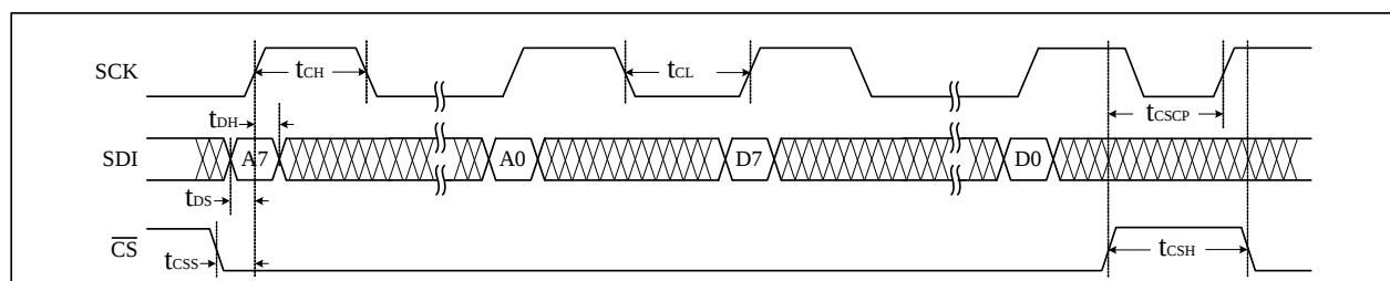
Figure 2 Interface Timing
