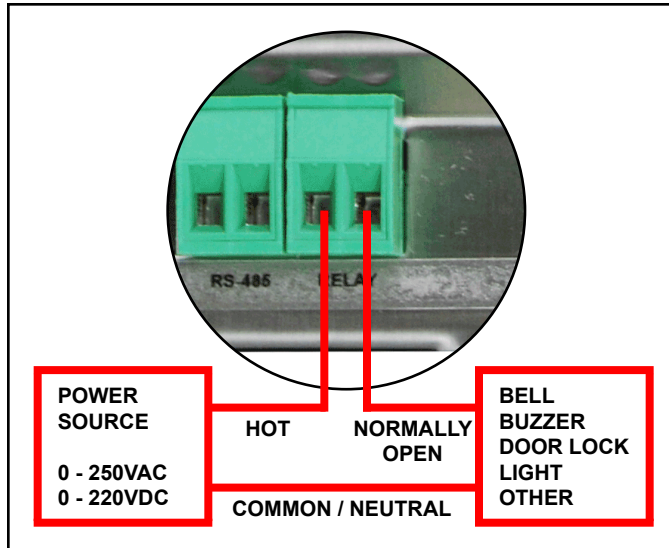
Figure 16. Relay installation
