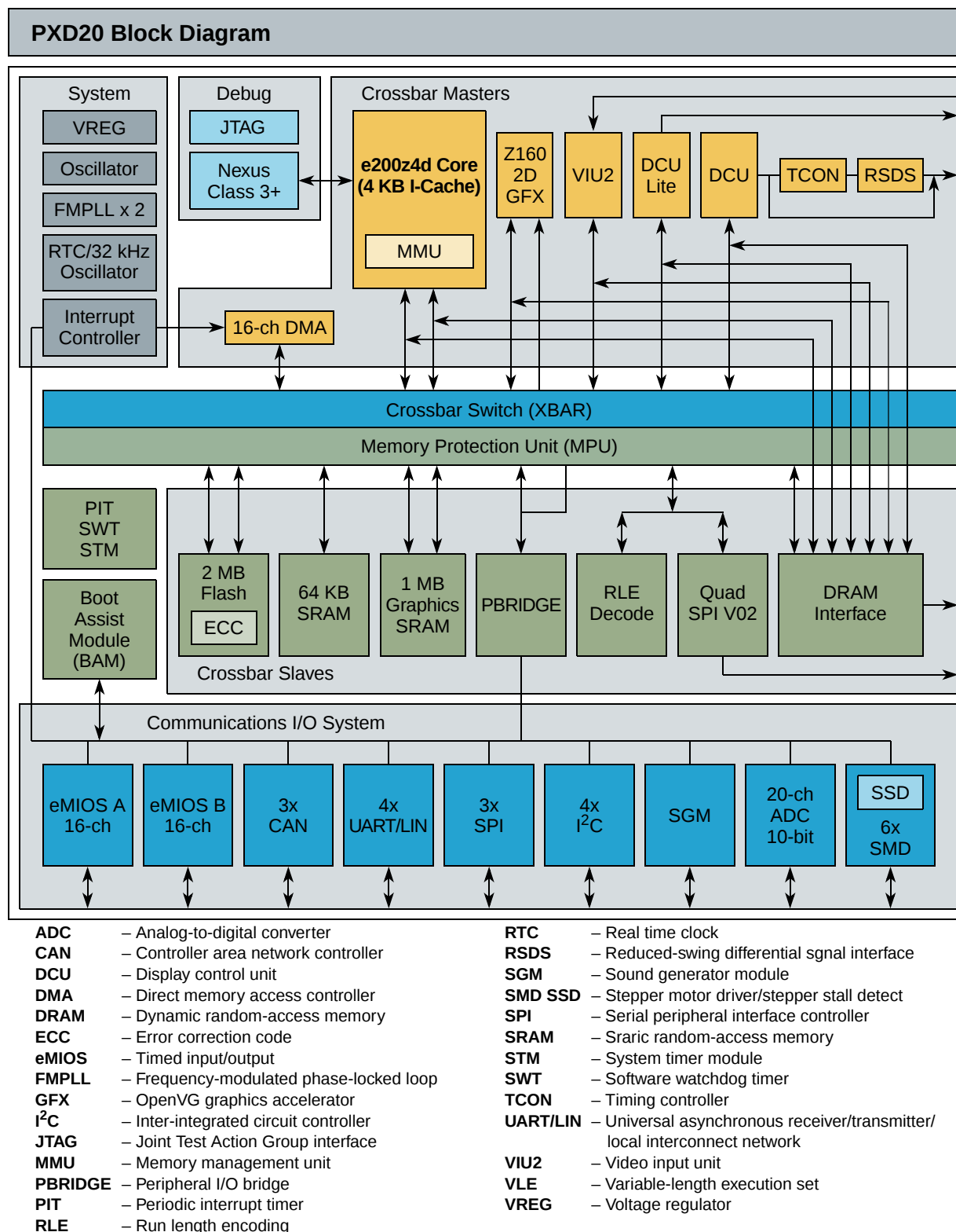
Figure 1. PXD20 block diagram
