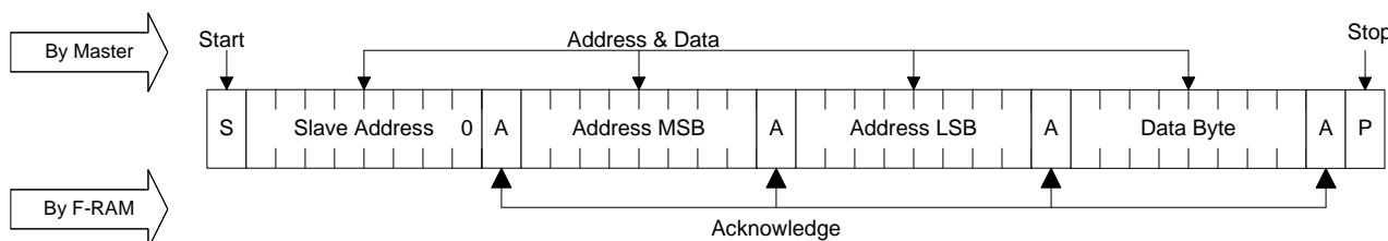
Figure 17. Single-Byte Write
