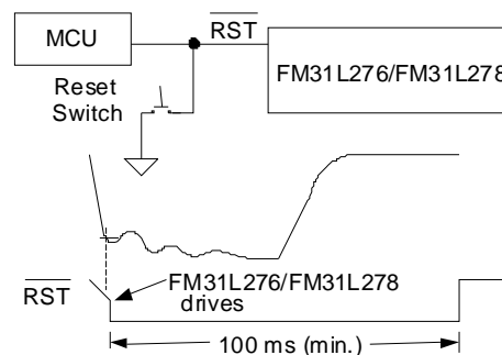
Figure 4. Manual Reset
