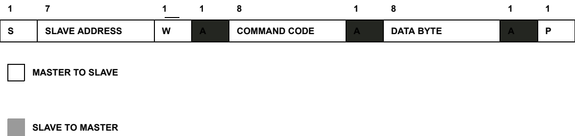
FIGURE 26. WRITE BYTE PROTOCOL
