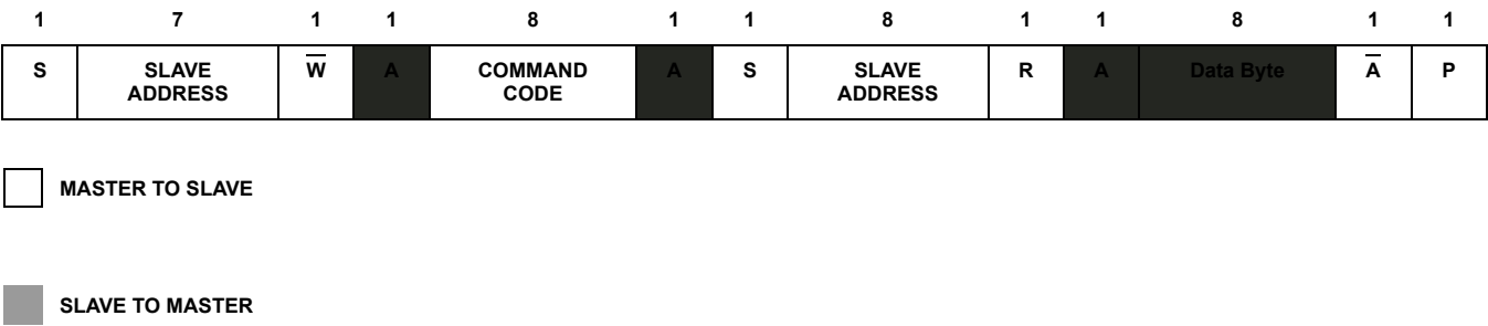
FIGURE 27. READ BYTE PROTOCOL
