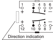
Schematic (Bottom view) 2 coil latching (L2)
