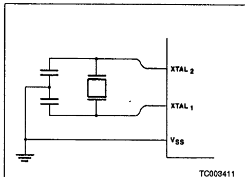
Figure 1. Crystal Oscillator
