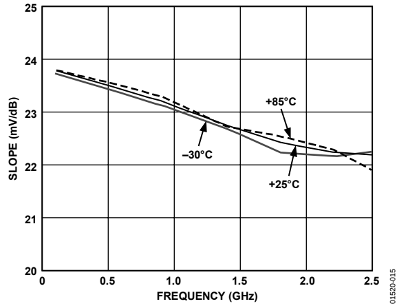
Figure 15. Slope vs. Frequency; -30°C, +25°C, and +85°C
