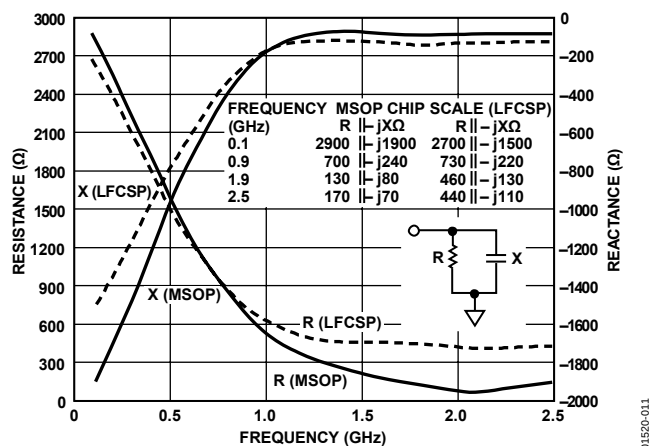
Figure 11. Input Impedance
