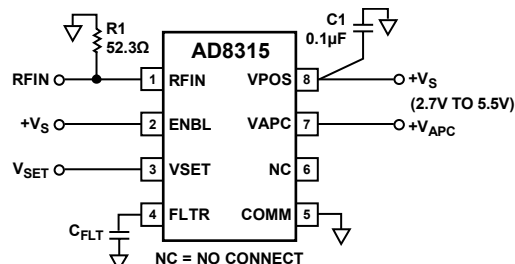
Figure 36. Basic Connections
