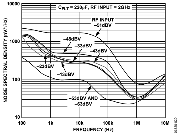
Figure 20. VAPC Noise Spectral Density
