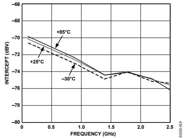
Figure 18. Intercept vs. Frequency; -30°C, +25°C, and +85°C
