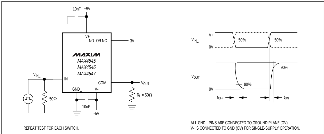
Figure 4. Switching Time
