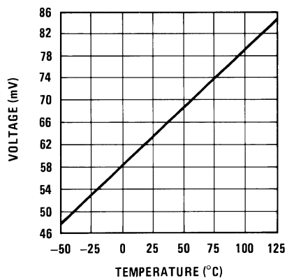
Voltage Across R_{\text{SET}} ( V_R )
