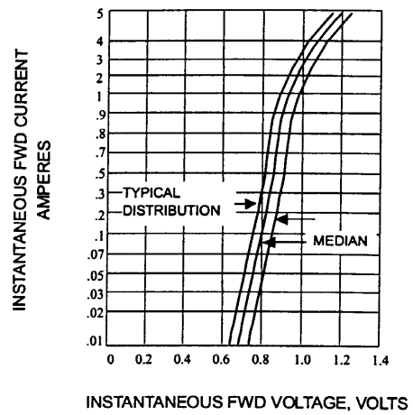
Fig. 2-TYPICAL FORWARD CHARACTERISTICS(25°C)
