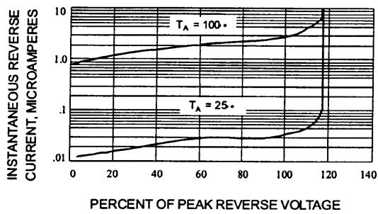
Fig. 3-TYPICAL REVERSE CHARACTERISTICS
