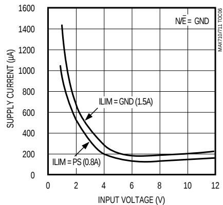
NO-LOAD BATTERY CURRENT vs. INPUT VOLTAGE
