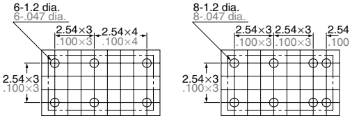
PC board pattern (Copper-side view) Single side stable
