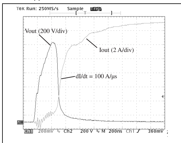
Fig. 4: Current and voltage of the ACS™ during IEC61000-4-5 standard test with a 150Ω - 10μH load & V_{DD} = 2kV .
