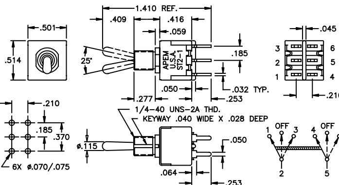
DOUBLE POLE
