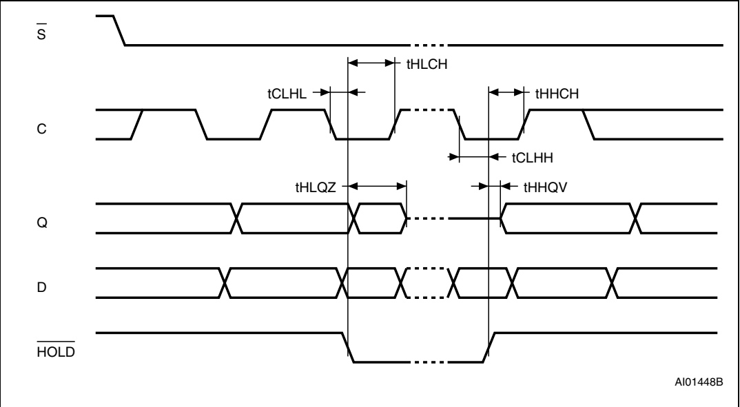
Figure 17. Hold timing
