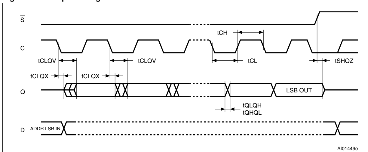
Figure 18. Output timing
