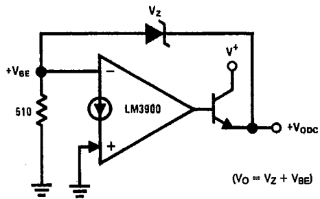
Voltage Regulator
