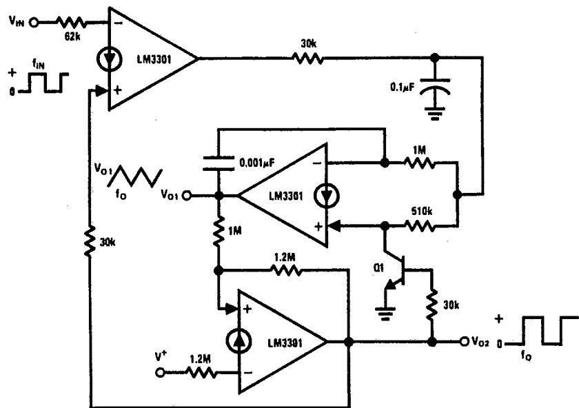
Phase-Locked Loop
