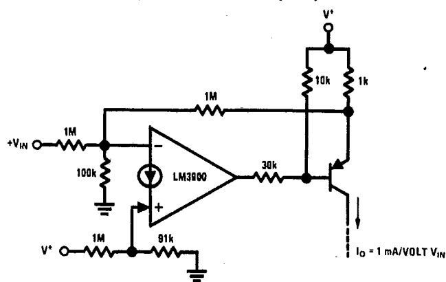
Voltage-Controlled Current Source (Transconductance Amplifier)
