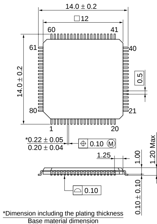
Figure G-2 Package Dimensions (TFP-80C)
