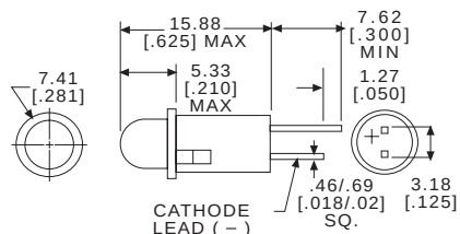
STRAIGHT TERMINALS - TERMINAL OPTION 1
