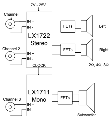
2.1 Audio Amplifier Configuration
