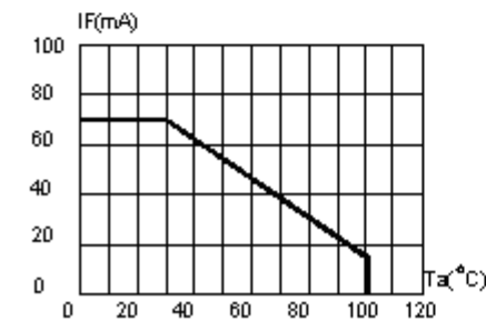
FIG.5 MAXIMUM FORWARD DC CURRENT VS. AMBIENT TEMPERATURE ( T_{jmax}=120\text{ }^{\circ}\text{C} )
