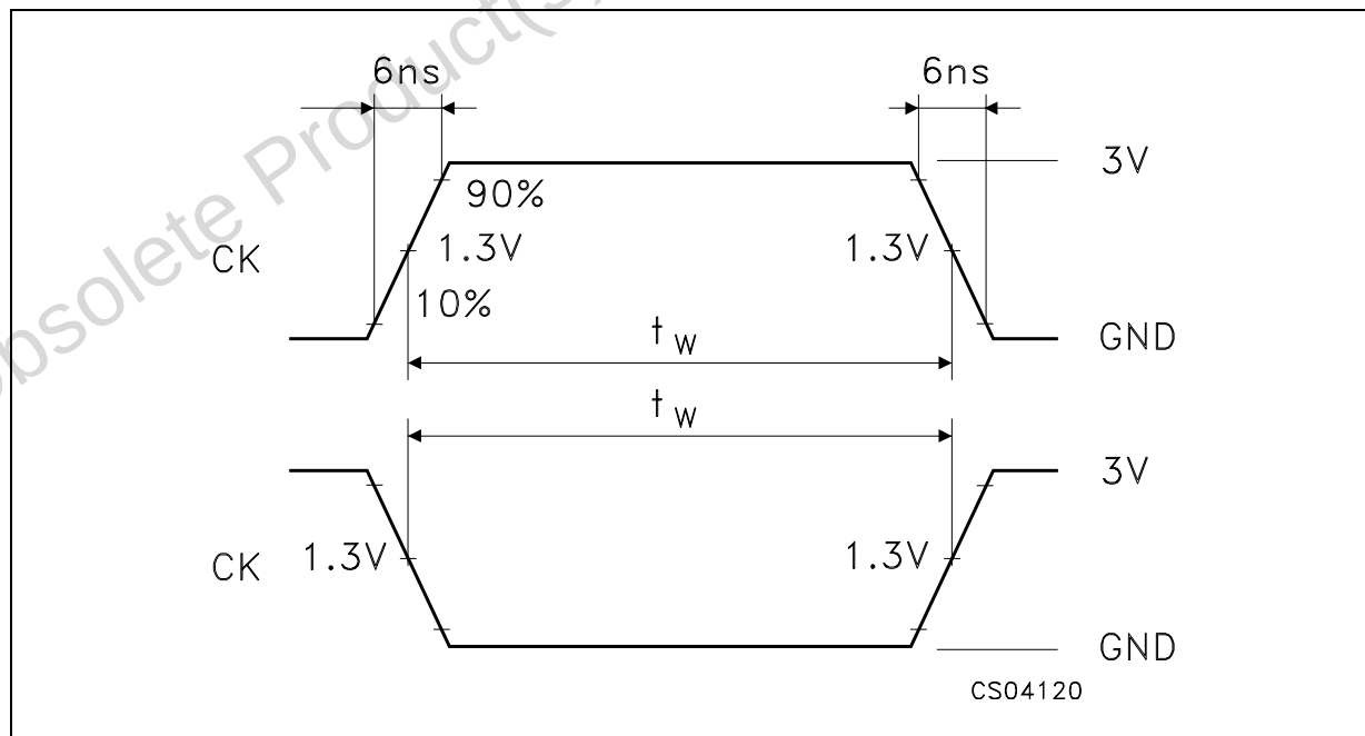
WAVEFORM 3 : MINIMUM PULSE WIDTH ( f=1\text{MHz} ; 50% duty cycle)
