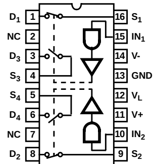
DUAL SPDT - DG190, DG191 (CDIP) TOP VIEW
