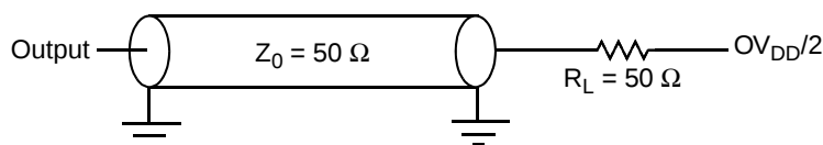
Figure 34. AC Test Load for the JTAG Interface
