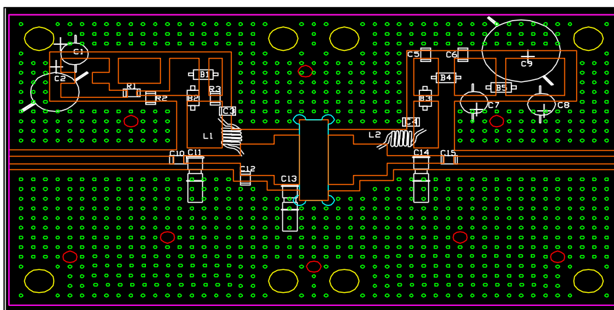
Figure 11. Circuit layout
