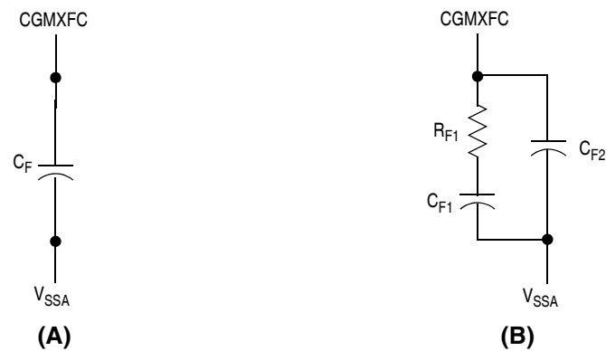
Figure 4-10. PLL Filter Table 4-4. Example Filter Component Values
