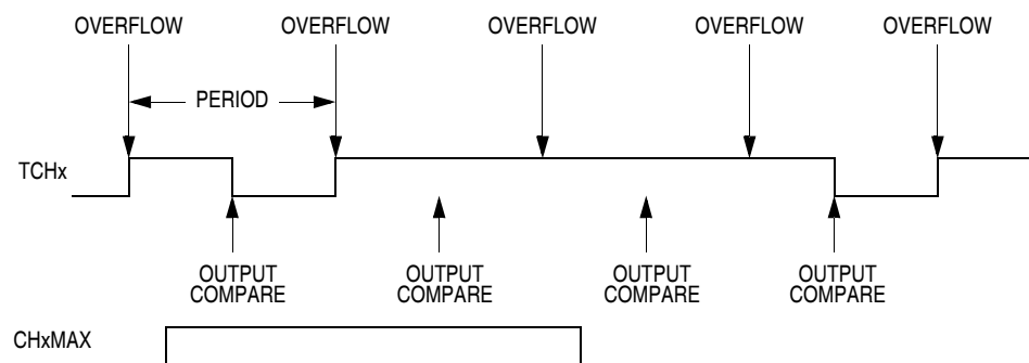
Figure 18-12. CHxMAX Latency
