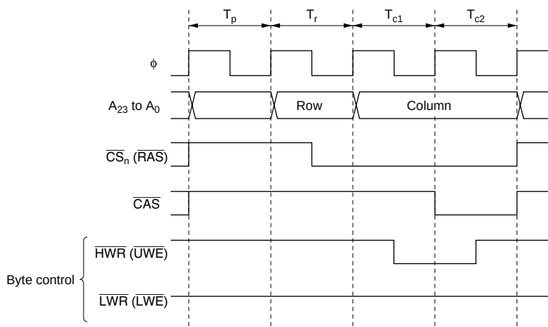
Figure 6.20 2-WE System Control Timing (Upper Byte Access)
