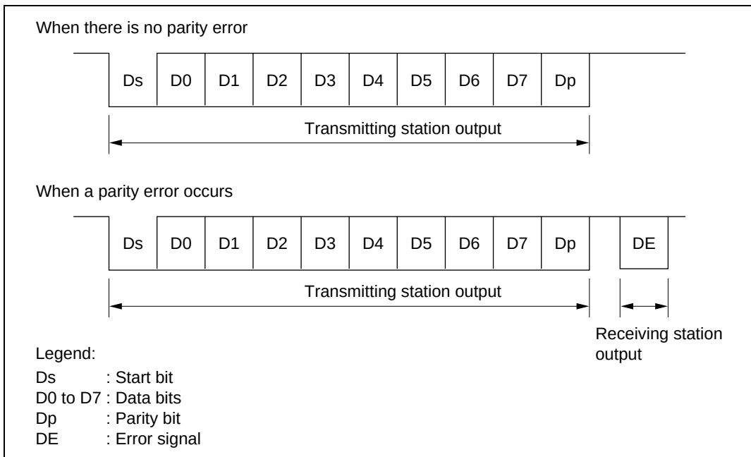
Figure 15.4 Smart Card Interface Data Format
