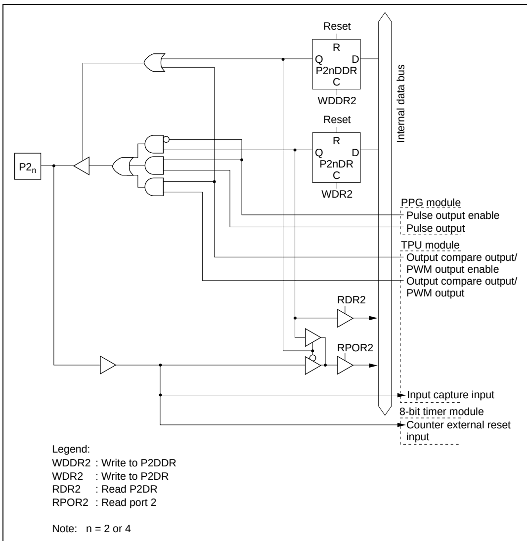
Figure C.2 (b) Port 2 Block Diagram (Pins P2_n and P2_n )
