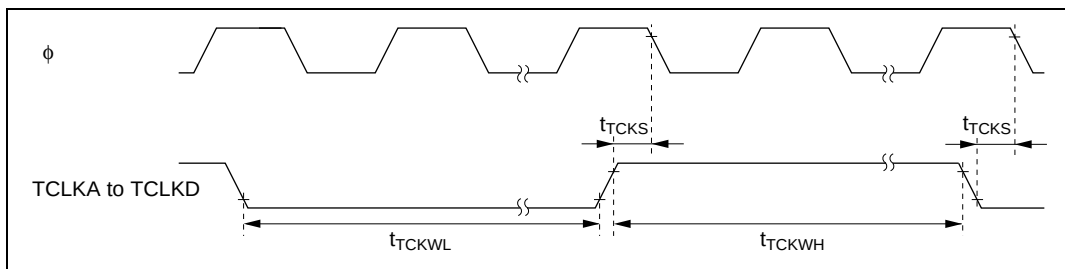
Figure 22.28 TPU Clock Input Timing
