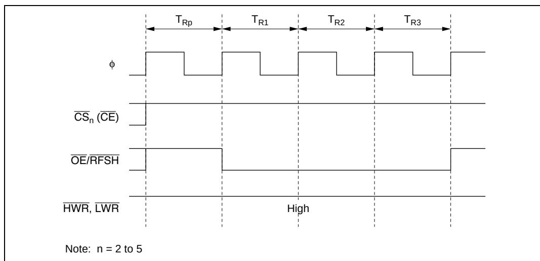
Figure 6.38 Auto-Refresh Timing
