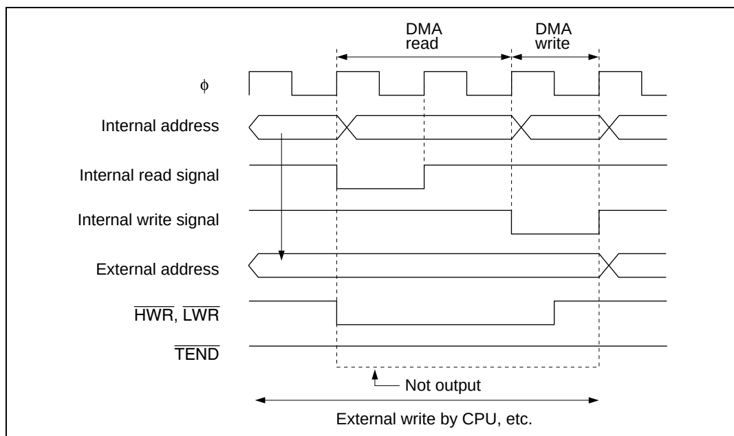
Figure 7.40 Example in Which Low Level Is Not Output at \overline{\text{TEND}} Pin
