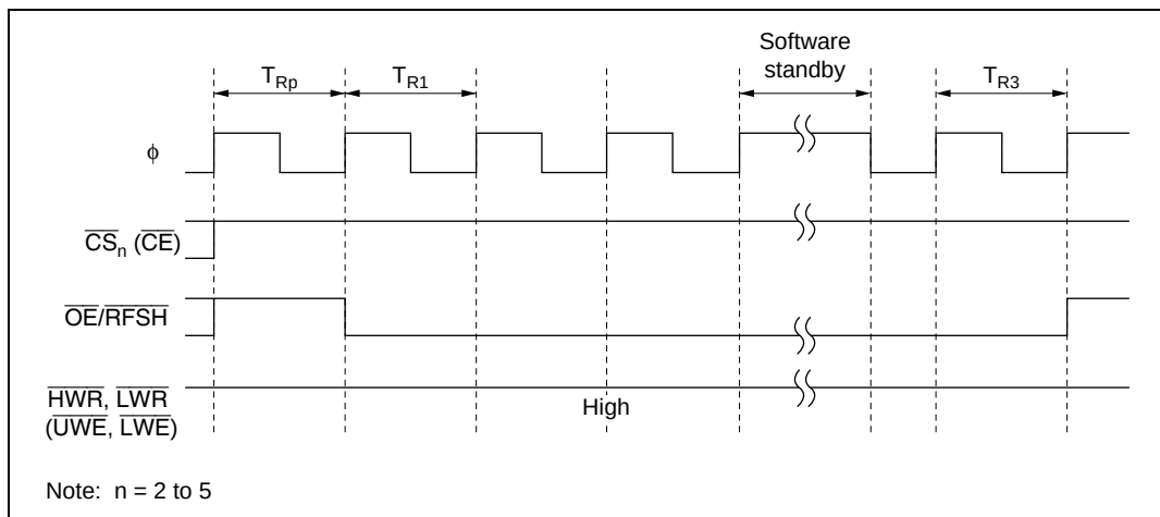
Figure 6.39 Self-Refresh Timing
