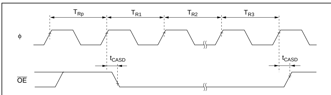
Figure 22.16 Self-Refresh Timing
