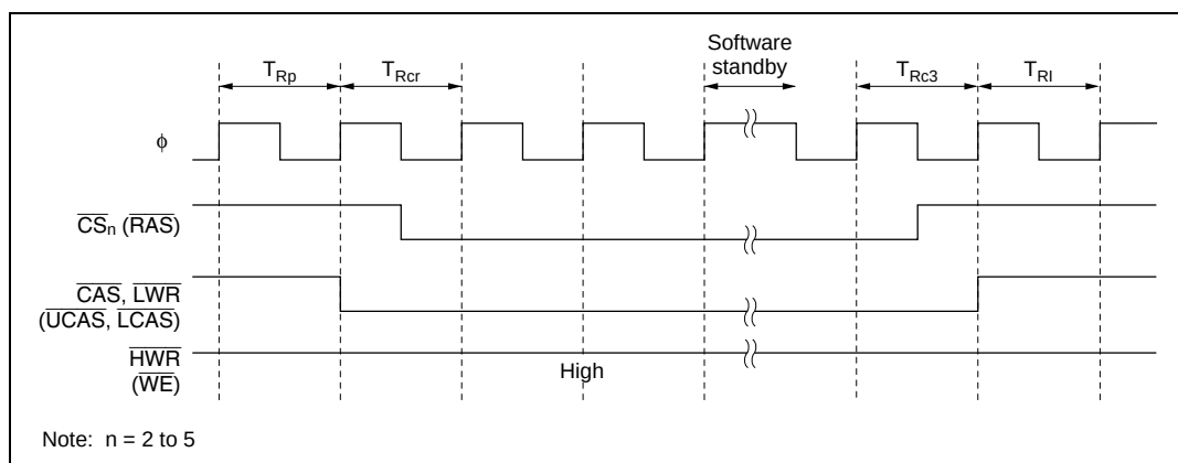
Figure 6.31 (b) Self-Refresh Timing (When CW2 = 0, LCASS = 1)
