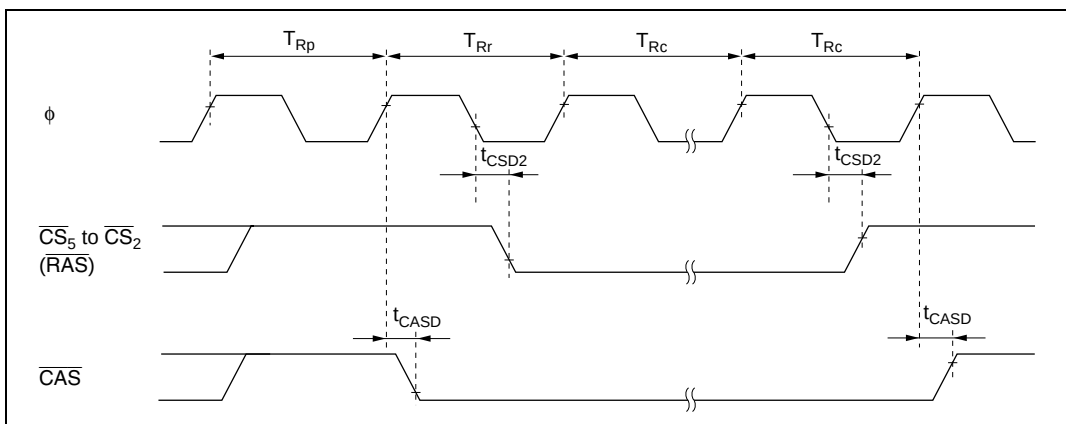
Figure 22.13 Self-Refresh Timing
