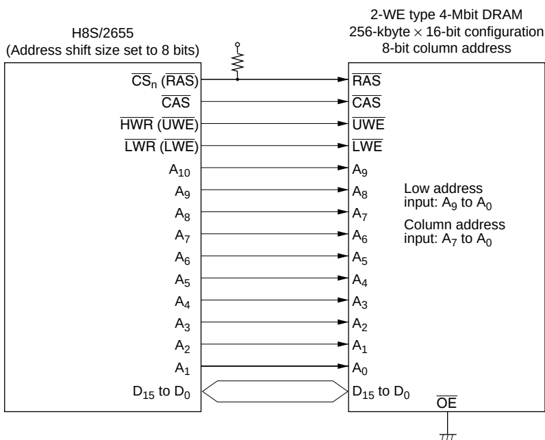
Figure 6.21 Example of 2-WE Type DRAM Connection
