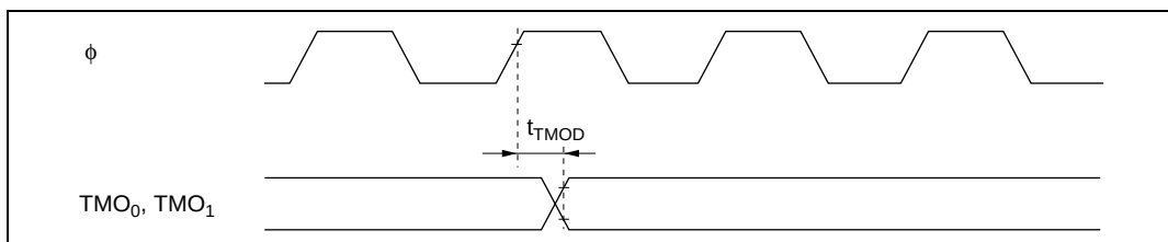
Figure 22.29 8-Bit Timer Output Timing
