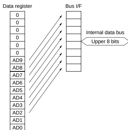
Figure 16.2 ADDR Read Operation
