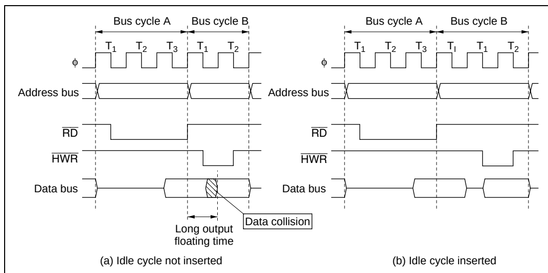
Figure 6.44 Example of Idle Cycle Operation (2) (When ICIS0 = 1)
