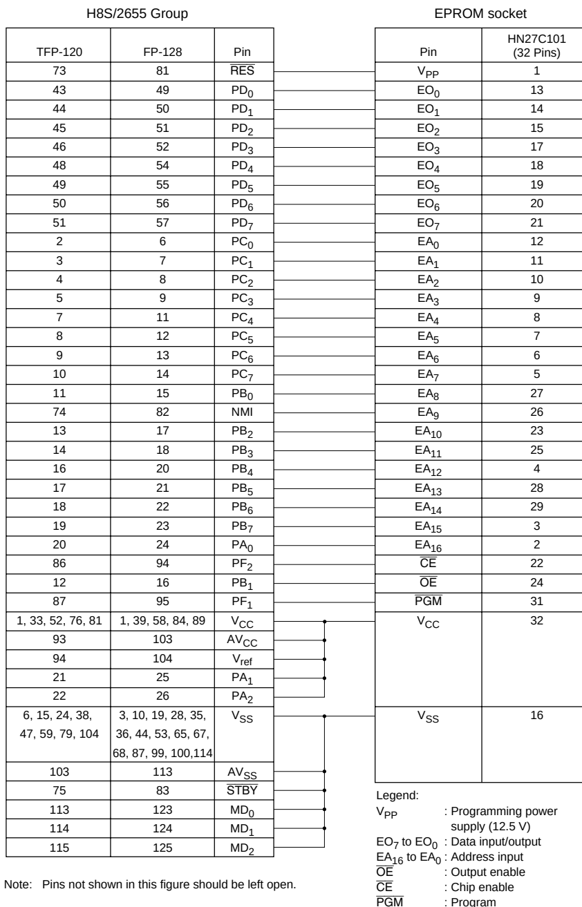
Figure 19.2 Wiring of 120-Pin/32-Pin Socket Adapter
