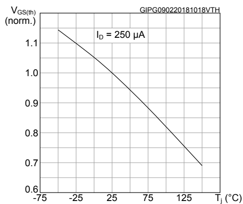
Figure 5. Normalized gate threshold voltage vs temperature
