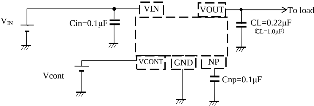
Figure 7. External Circuit
