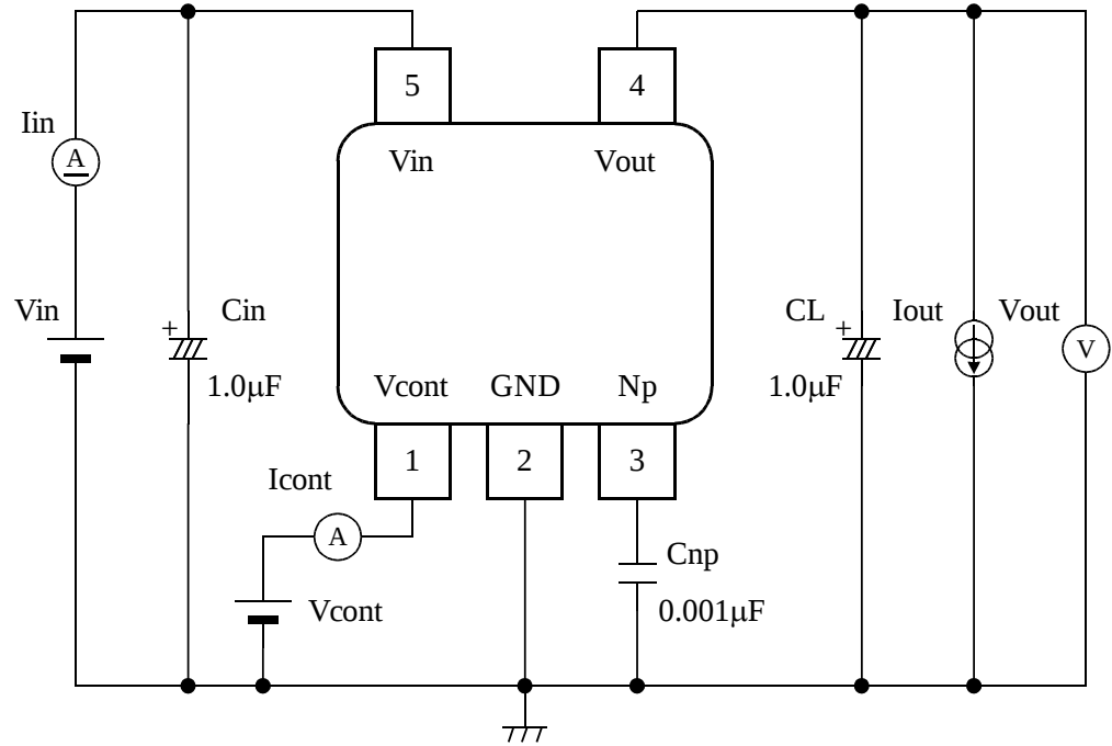
Figure 8. Test Circuit
