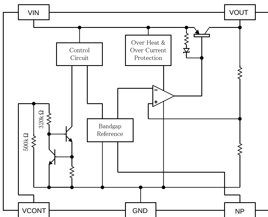
Figure 1. Block Diagram
