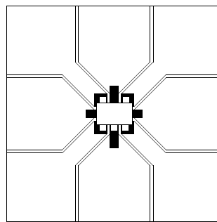
Figure 5. Example PCB layout
