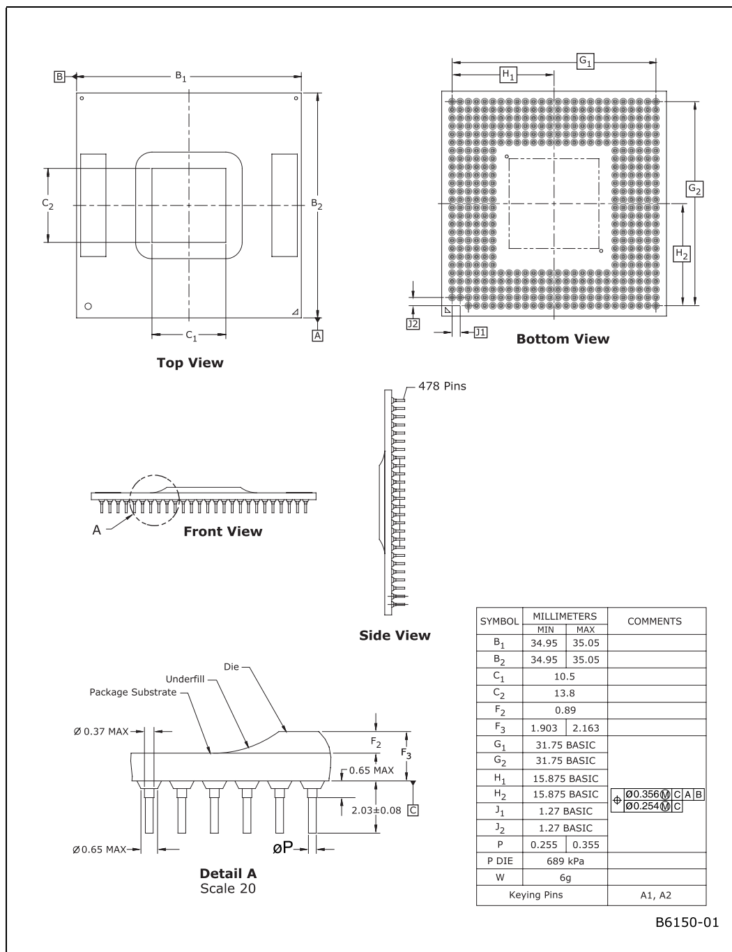
Figure 5. 1-MB Fused Micro-FCPGA Processor Package Drawing (1 of 2)
