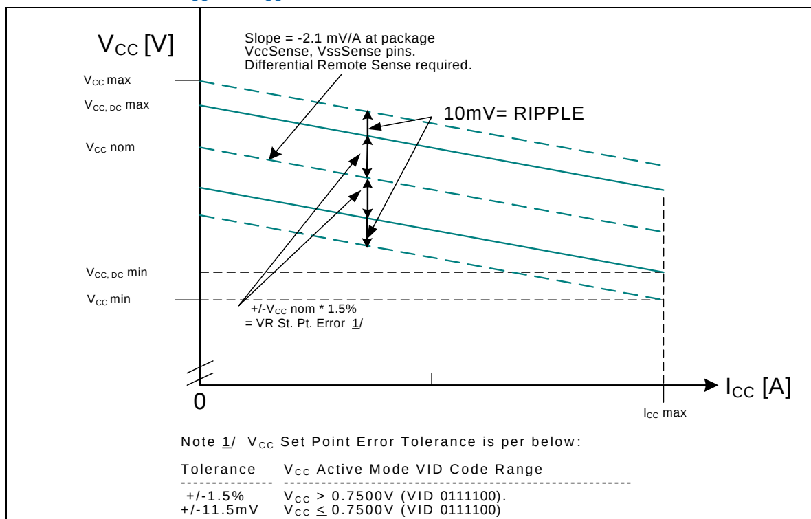
Figure 3. Active V_{CC} and I_{CC} Loadline Standard Voltage
