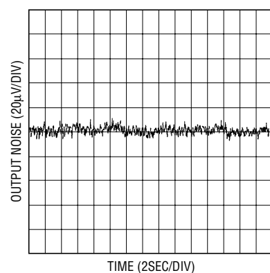
Output Noise 0.1Hz ≤ f ≤ 10Hz
