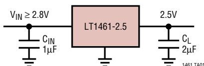
Basic Connection
