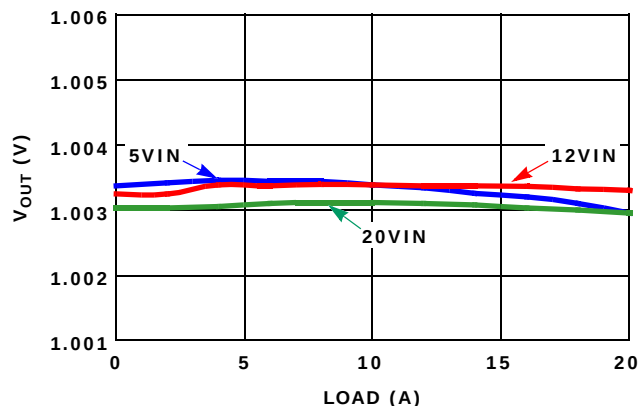
FIGURE 11. LOAD REGULATION (5, 12, 20V IN )
