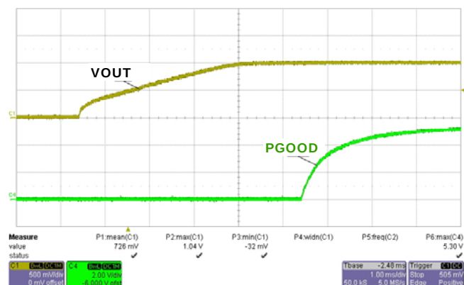
FIGURE 12. START-UP UNDER NO LOAD, PVIN = V IN = 12V, I OUT = 0A
