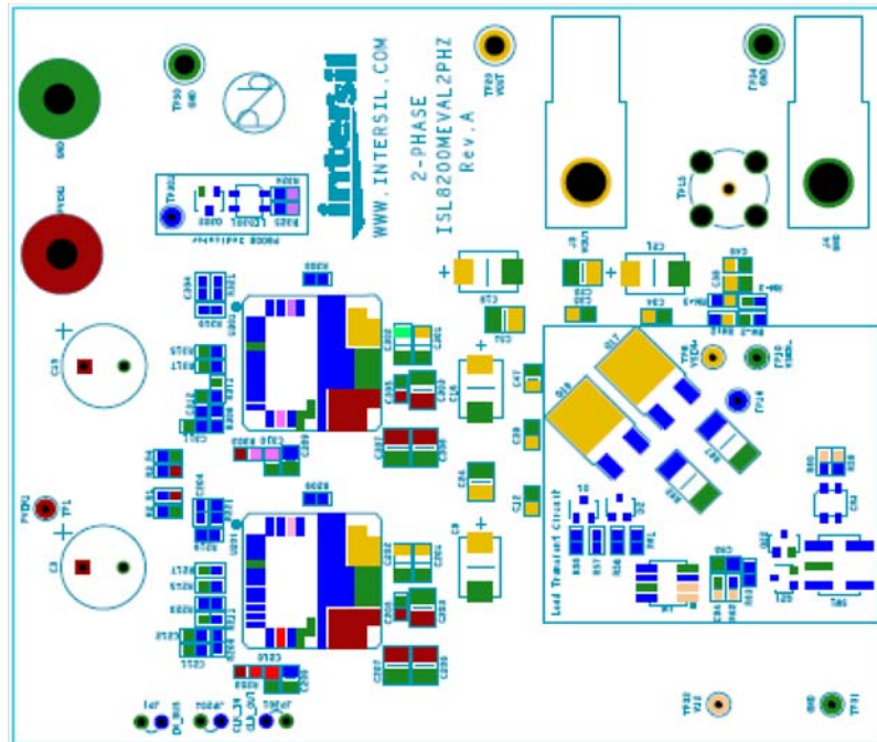
FIGURE 4. TOP COMPONENTS
