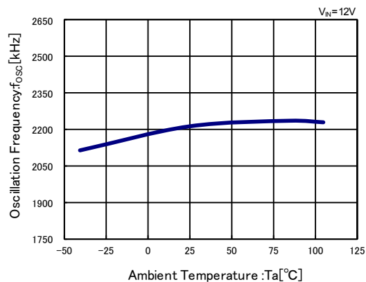
XC9263x75D/XC9264x75D ( f_{osc}=2200\text{kHz} )
