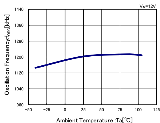
XC9263x75C/XC9264x75C ( f_{osc}=1200\text{kHz} )
