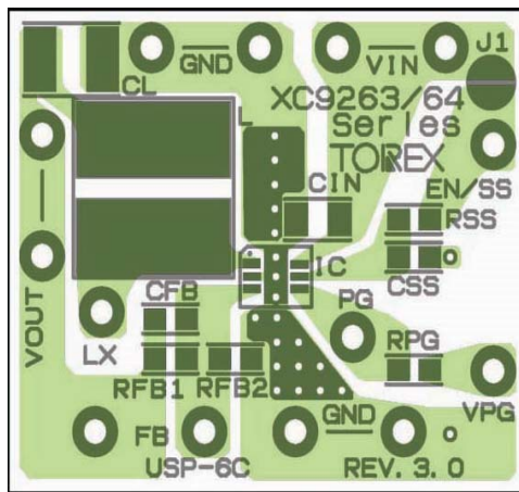
USP-6C (Front)
