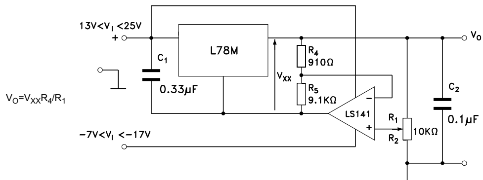
Figure 21. 0.5 to 10 V regulator
