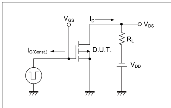
図 4-1 GATE CHARGE MEASUREMENT CIRCUIT
