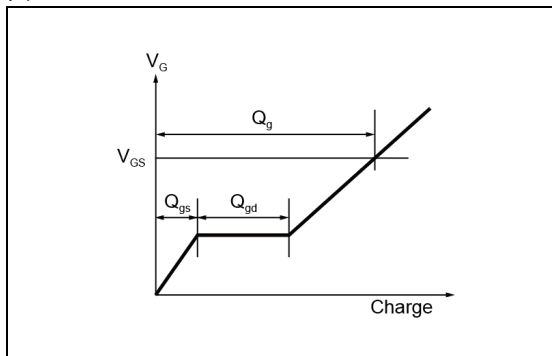
図 4-2 GATE CHARGE WAVEFORM
