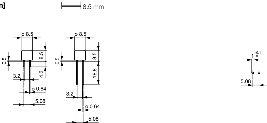
Drilling diagram
