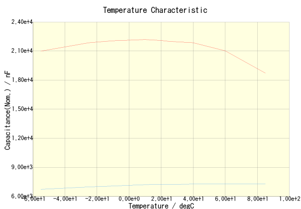
C2012X5R1A226K125AB(DC Bias = 0V) C2012X5R1A226K125AB(DC Bias = 5V)
