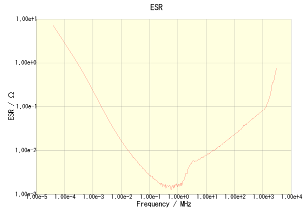
C2012X5R1A226K125AB
