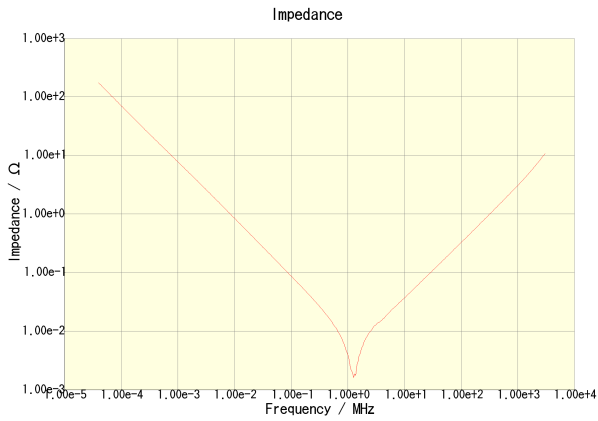
C2012X5R1A226K125AB
