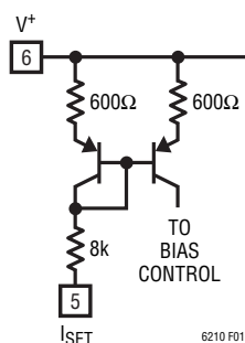
Figure 1. Internal Bias Setting Circuitry
