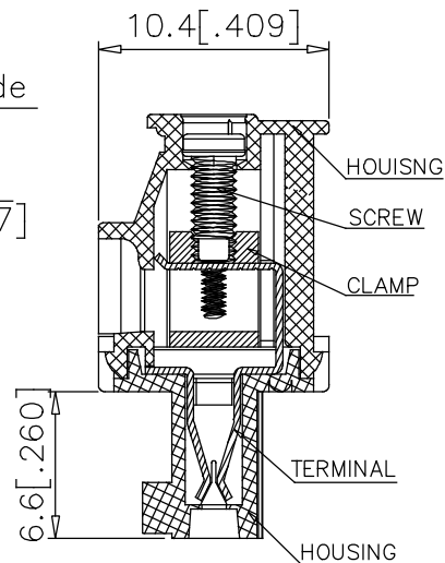
SECTION P-P
