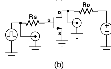
(a) I_D^{\text{MAX}} measurement scheme R=1\Omega , C=100\mu\text{F} , Compliance ( V_{DS}=80\text{V} )=100mA (b) Timing measurement scheme R_G=0\Omega , R_D=15\Omega , V_{DS}=40\text{V} .
