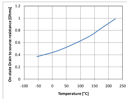
On-state drain source resistance vs. junction temperature ( V_G = 5\text{V} , V_D = 50\text{mV} ).
