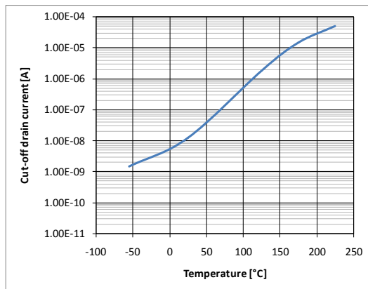
Cut-off current vs. junction temperature ( V_G = 0\text{V} , V_D = 80\text{V} ).
