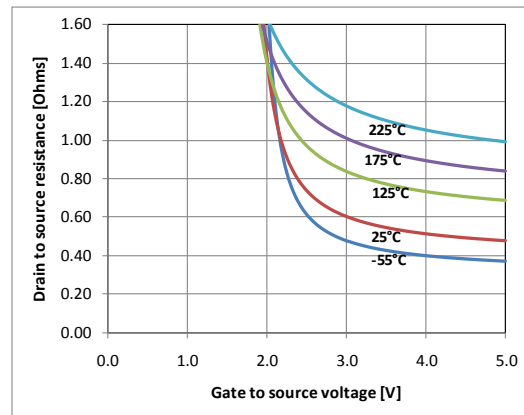
Drain-source resistance vs. gate voltage ( V_D = 50\text{mV} )
