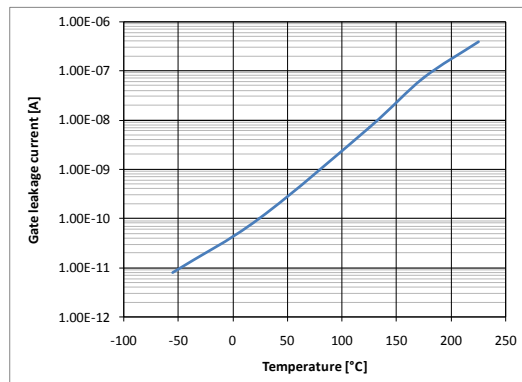
Gate and ESD diode leakage current vs. junction temperature ( V_G = 5\text{V} , V_D = 50\text{mV} ).
