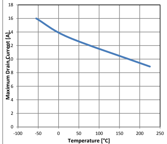
Peak drain current vs. temperature ( V_G=5\text{V} , V_D=80\text{V} ).
