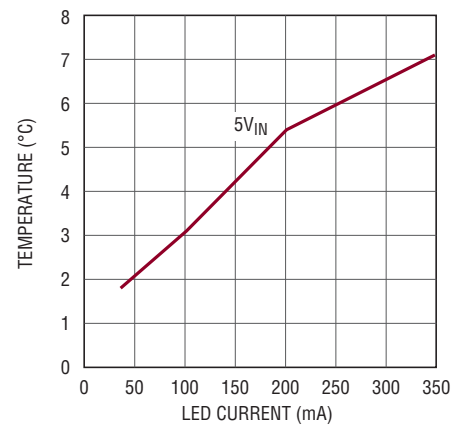
Junction Temperature Rise vs Load, Boost Operation, 11.2V at 350mA LED String
