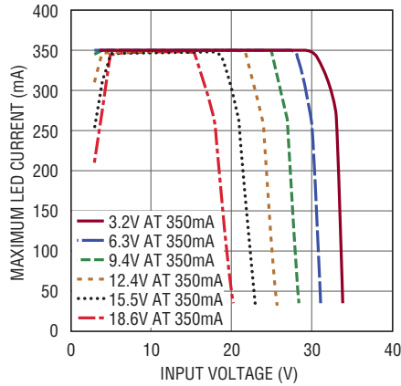
Maximum LED Current vs Input Voltage, Buck-Boost Mode
