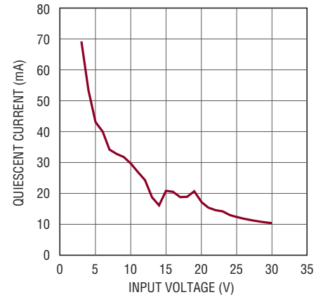
Quiescent Current vs Input Voltage, Open LED
