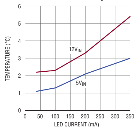
Junction Temperature Rise vs Load, Buck Mode, 3.2V at 350mA LED String
